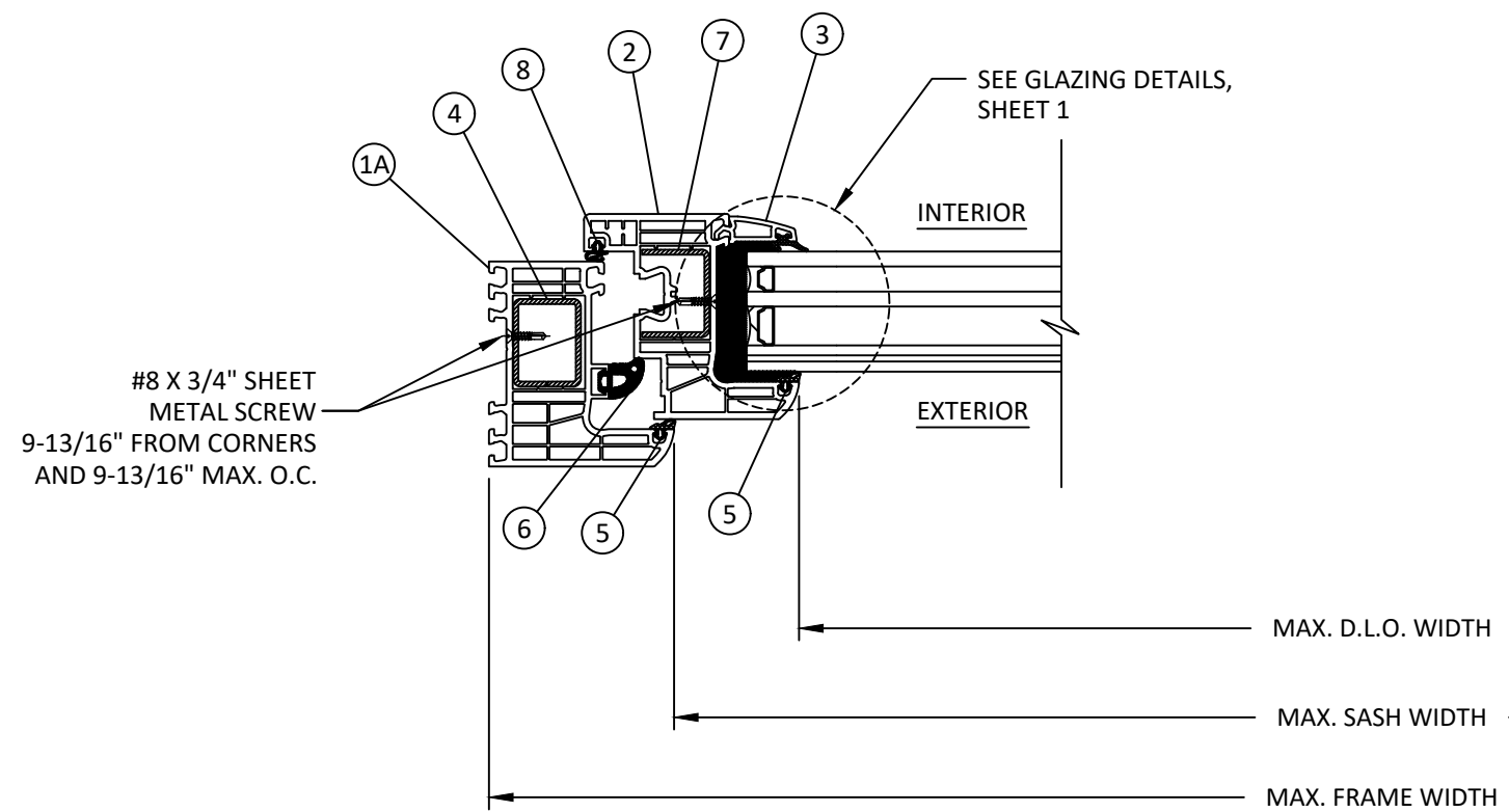
D HORIZONTAL SECTION 5 FINLESS SECTION DETAIL
