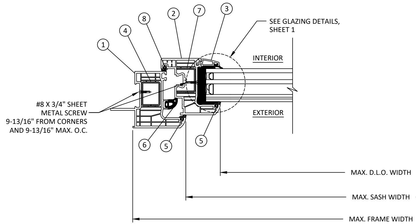
C HORIZONTAL SECTION 5 FIN SECTION DETAIL
