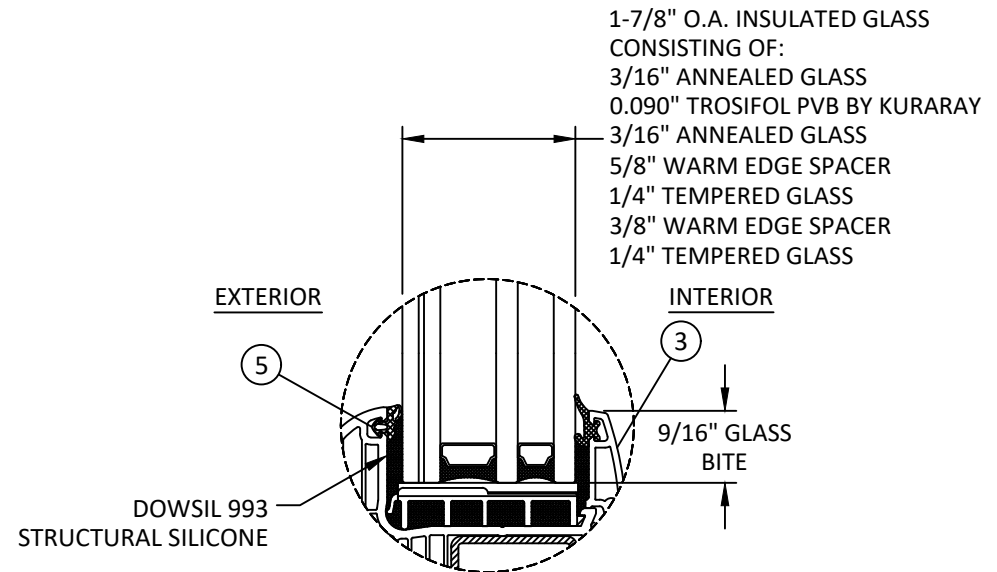
GLAZING DETAIL 1
