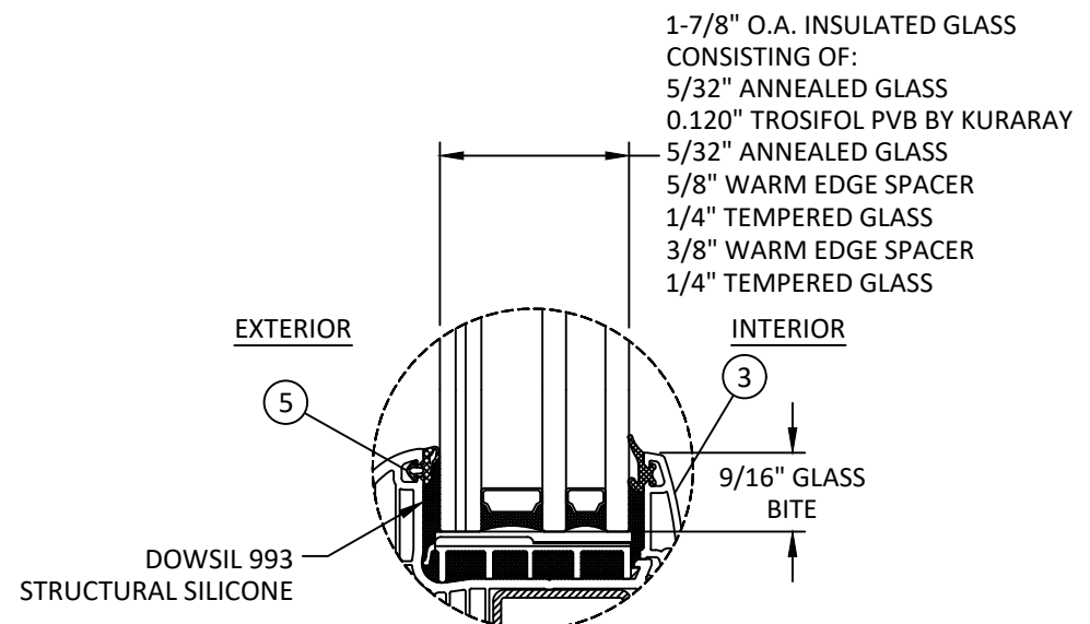
GLAZING DETAIL 2
